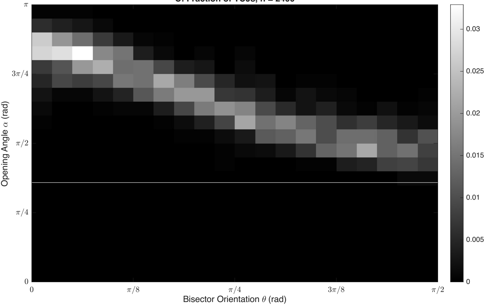
C: Fraction of TCJs, n = 2400
